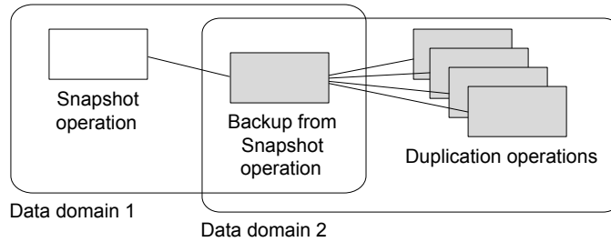
Figure 21-8 Hierarchical operations
