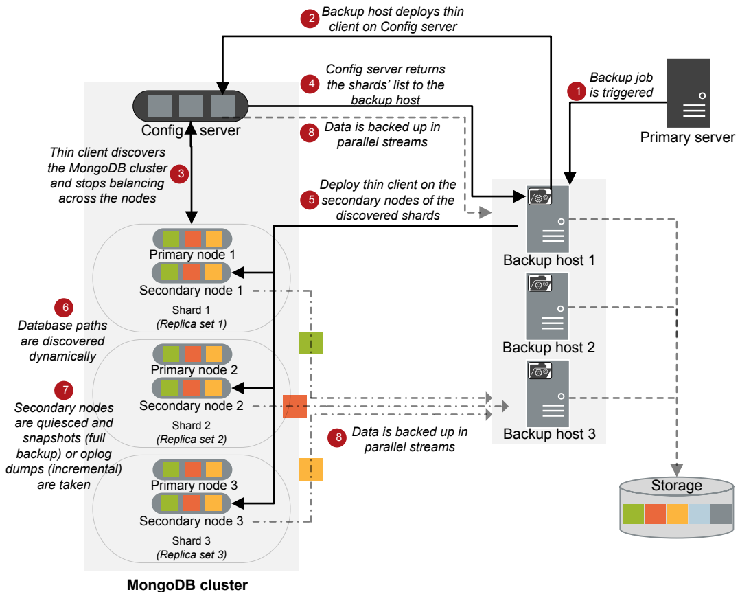
Figure 4-1 Backup flow
