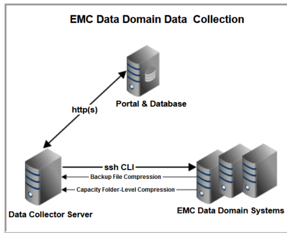
Figure 2 Data Collector in an EMC Data Domain Environment
