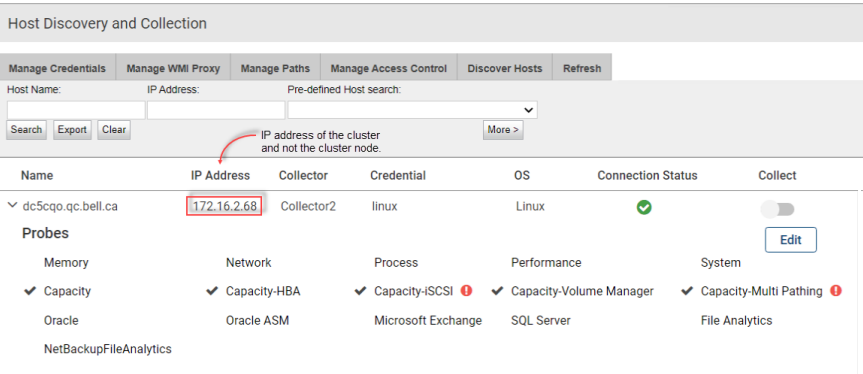
Figure 34-2 Application Probe Example
