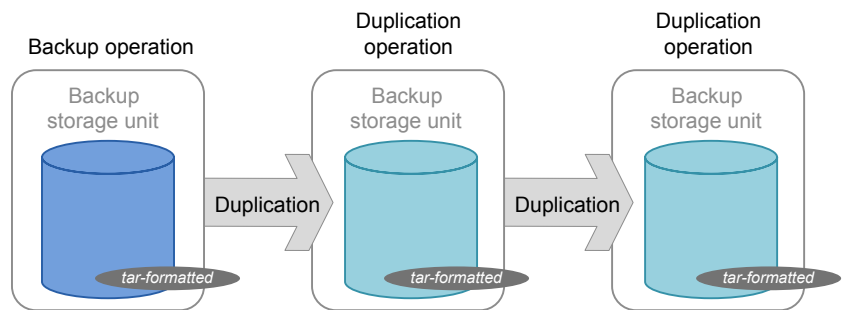
Figure 15-3 SLP that contains one Backup operation and two Duplication operations
