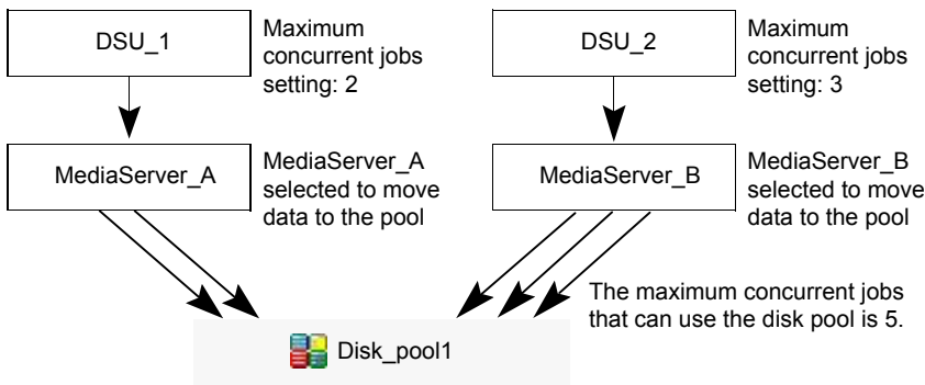
Figure 11-3 Impact when disk storage units use one disk pool but different media servers
