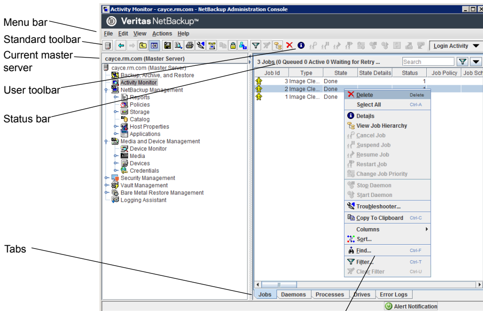
Figure 28-1 Activity Monitor
