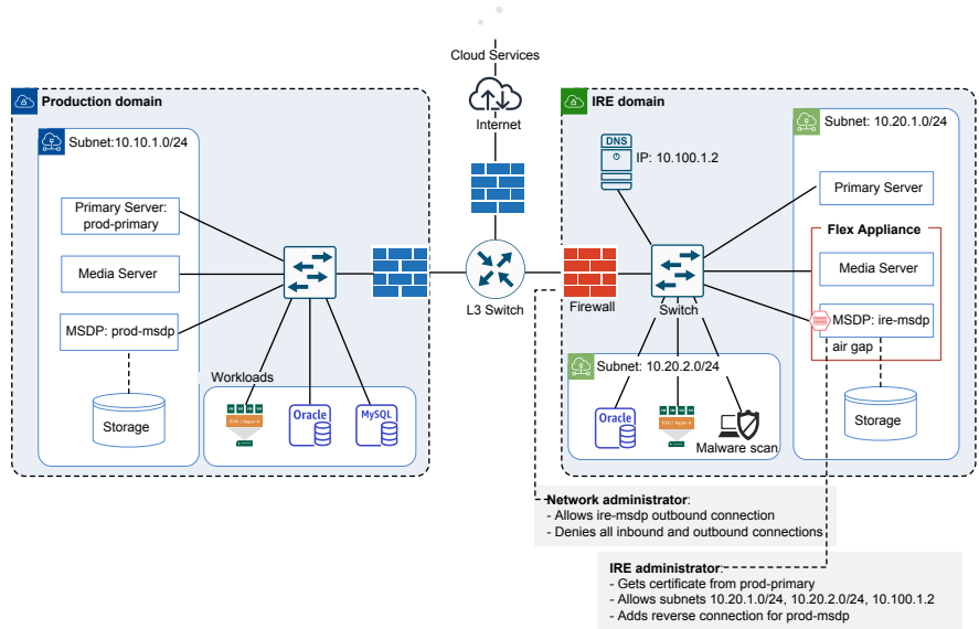
Figure 16-1 Network isolation example
