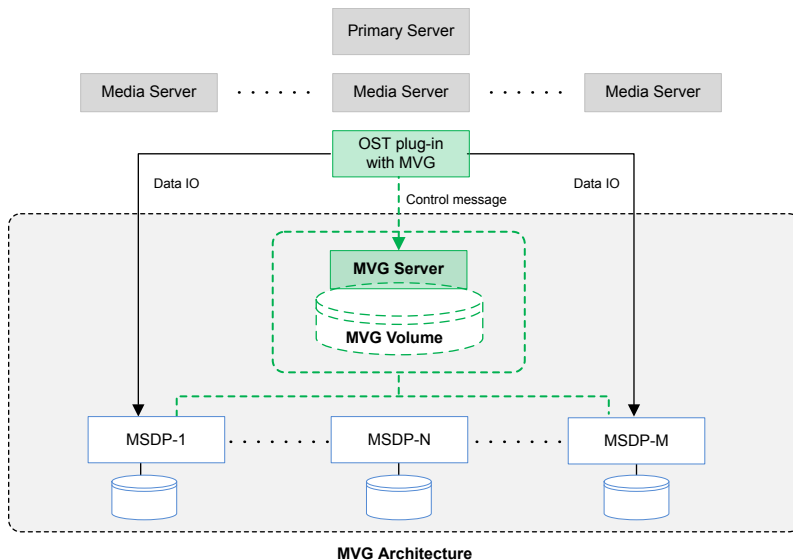
Figure 5-1 MVG architecture
