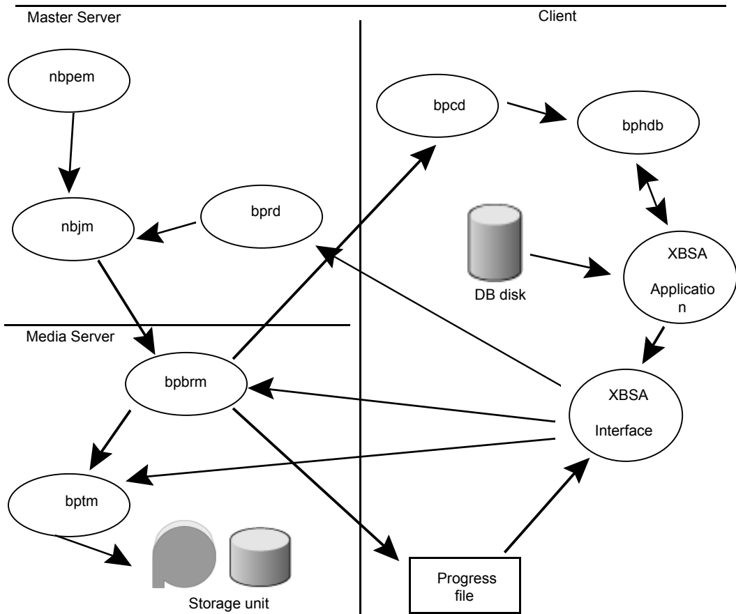
Figure 7-1 Stream backup process flow diagram
