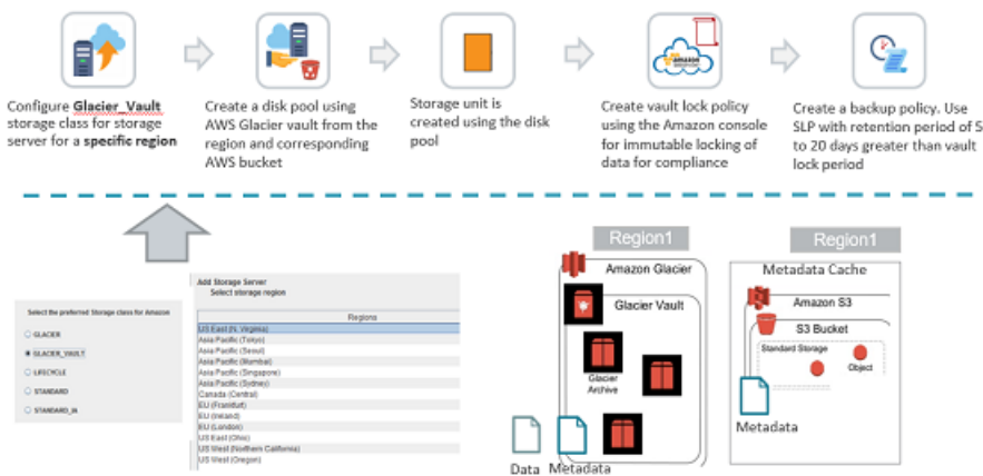
Figure 2-4 Protecting data in Amazon Glacier vault
