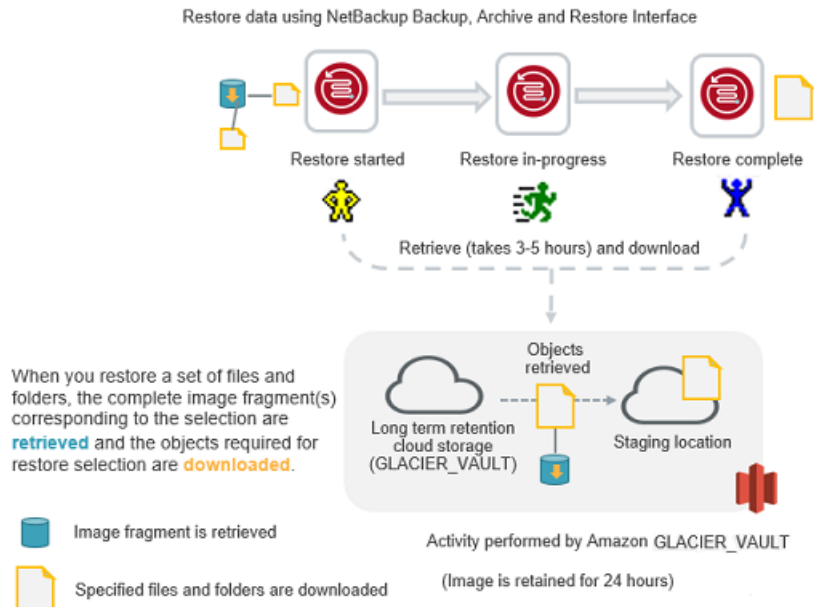
Figure 2-5 Restoring from Amazon Glacier vault
