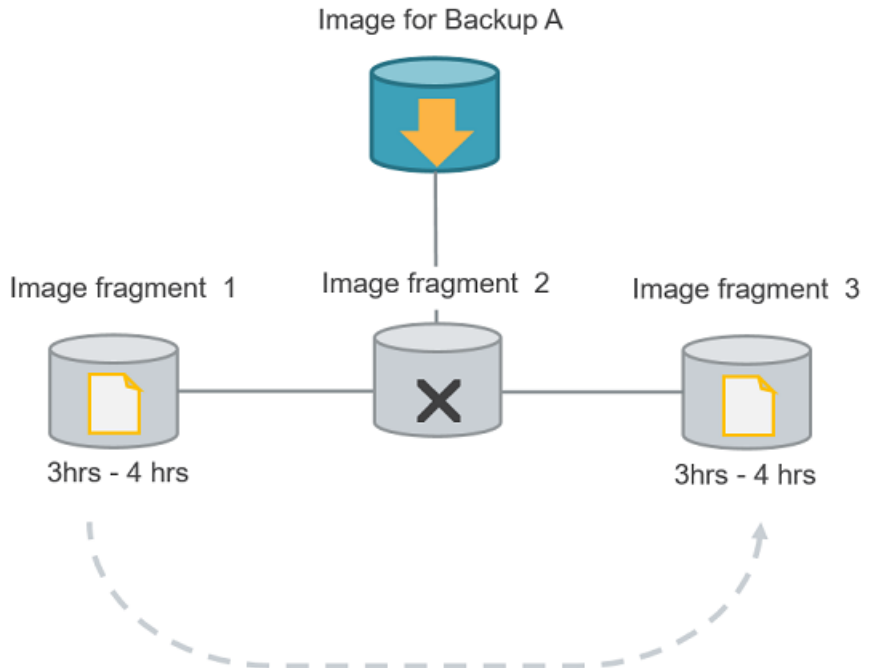
Figure 2-2 Restoring image fragments for Amazon Glacier
