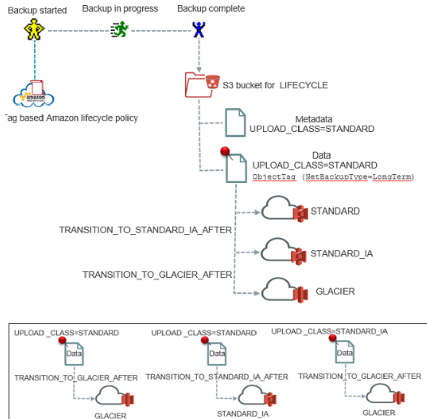
Figure 2-7 Back up process for Amazon S3 Intelligent Tiering (LIFECYCLE) storage class with possible configurations
