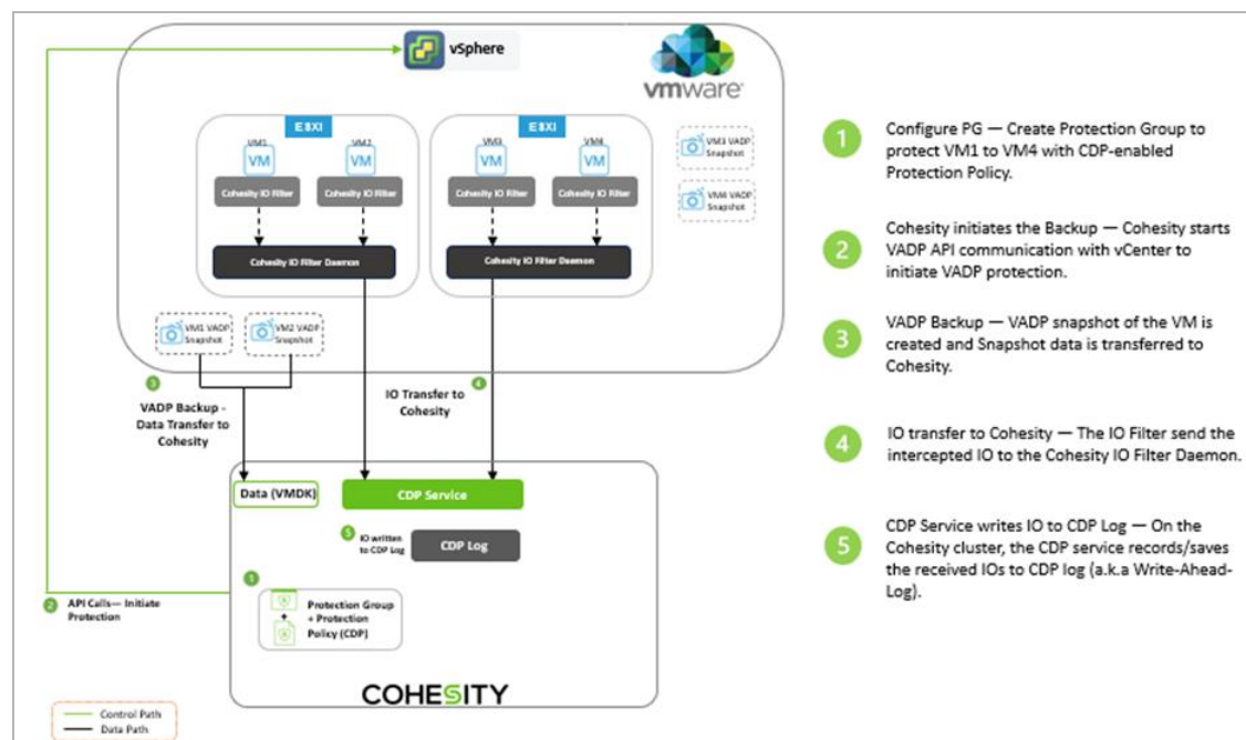
Figure 7: Cohesity Continuous Data Protection
