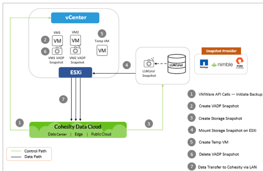
Figure 5: VM Backup Workflow - NBDSSL & Storage Snapshot
