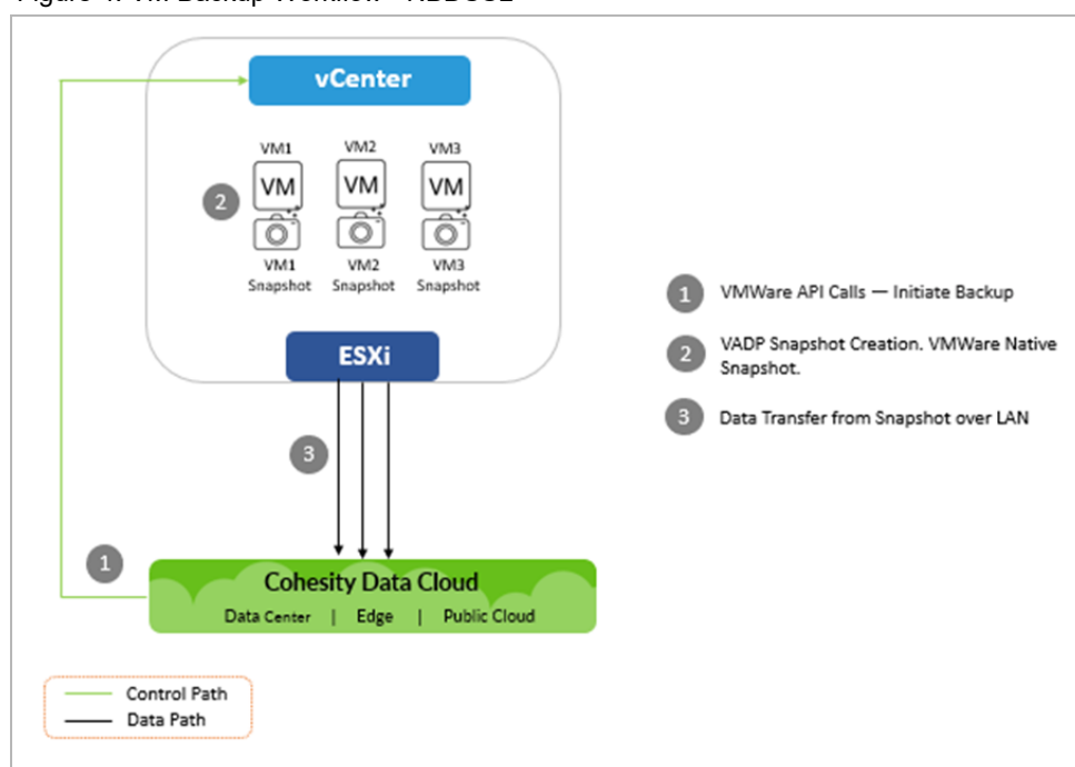
Figure 4: VM Backup Workflow - NBDSSL
