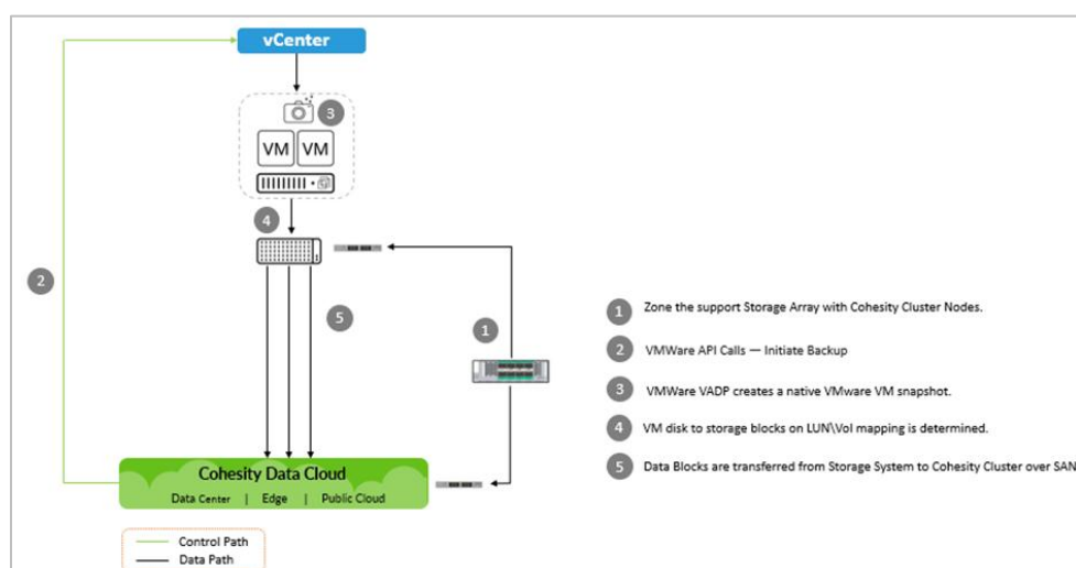
Figure 6: VM Backup Workflow - SAN Transport
